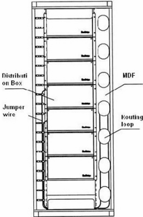
Picture7 Jump Wire Diagram Of This Frame
