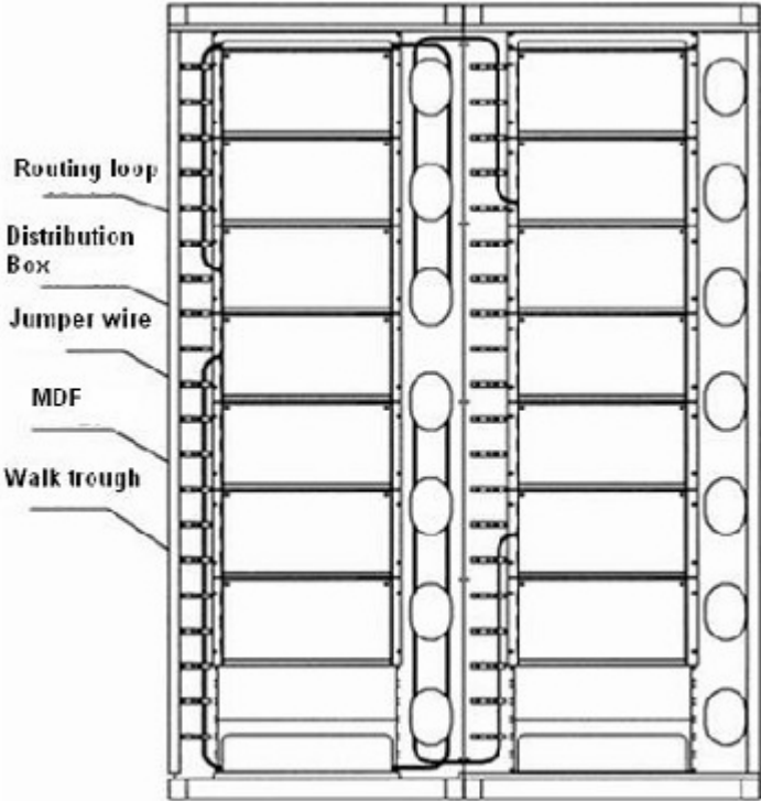
Picture8 Jump Wire Diagram Of Cross Frame
