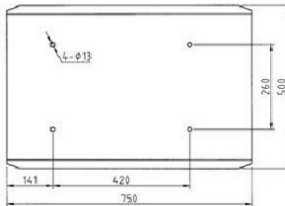
Picture4 Mounting Hole Diagram
