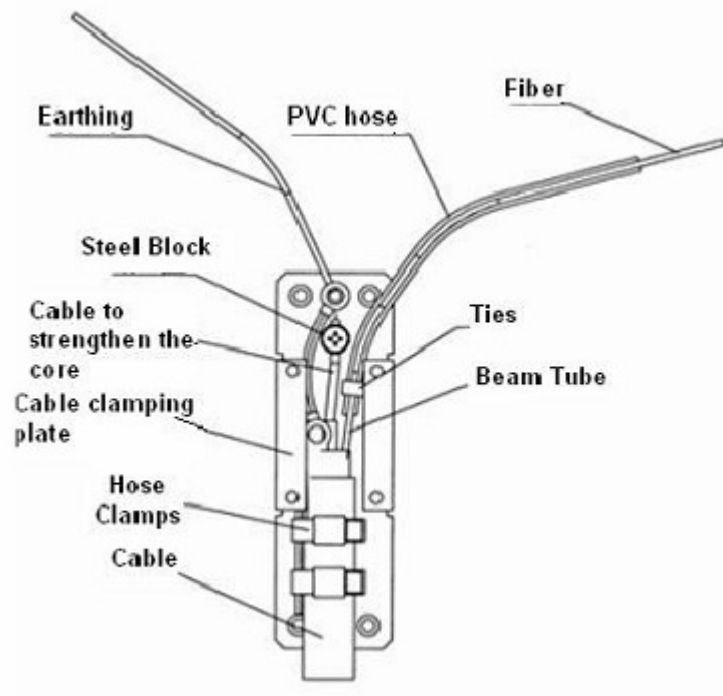
Picture4 Cable Peeling And Fixed
