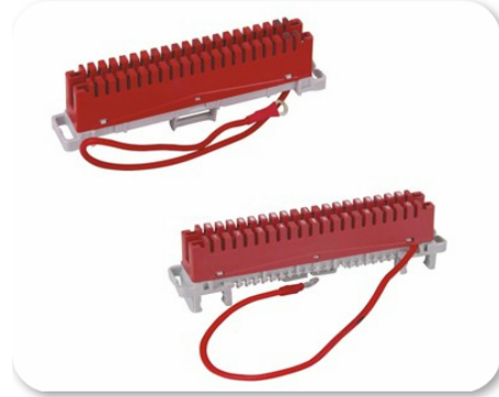
10 Pair Earth Module LSA-Plus LSA-Profile Item Code: STEM
