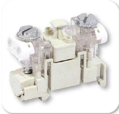
1 Pair Terminal Block STB Module Item Code:ST VX-MD01
