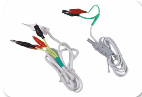
Test Cord 2 Pole 4 Pole Plug To Alligator Clip Item Code:STTC03
