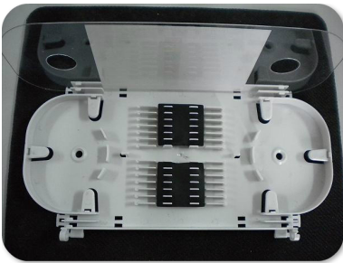
Fiber Optic Splice Tray 12 Core Item Code:STST02
