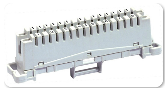
Disconnection/Connection Module 8 Pair LSA-Plus Item Code:STDM-8P STCM-8P
