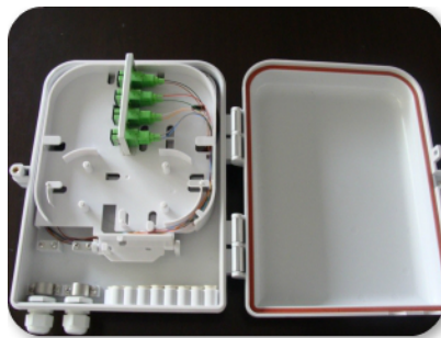
Outdoor Fiber Optic Distribution Box With 16 Core PLC Splitter Item Code STOFB02
