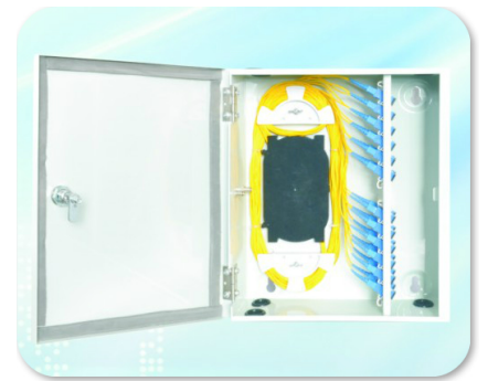
Indoor Fiber Optic Distribution Box With 16 Core PLC Splitter Item Code STIFB06
