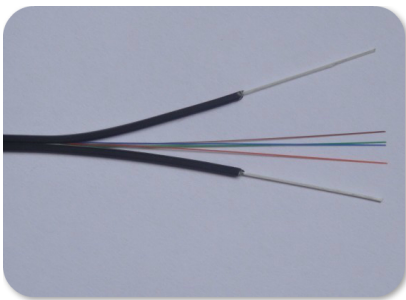
FTTH Drop Cable Item Code: STFTTHDC
