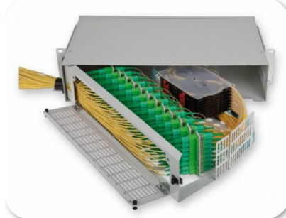
Fiber Optic Splice Patch Panels 12~96 Core Rotation Type Item Code:STFU10
