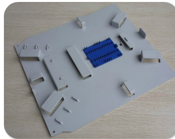
Fiber Optic Splice Tray 12 Core Item Code:STST03
