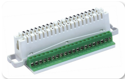
Disconnection Module With Screw Terminal Item Code:STDM-10PT
