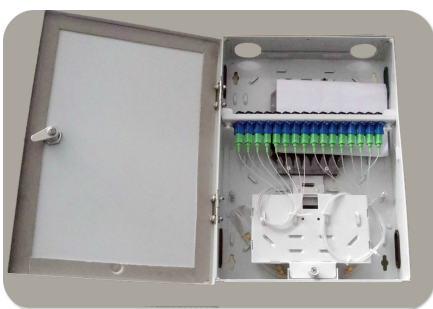
Indoor Fiber Optic Distribution Box With 16 Core PLC Splitter Item Code STIFB04
