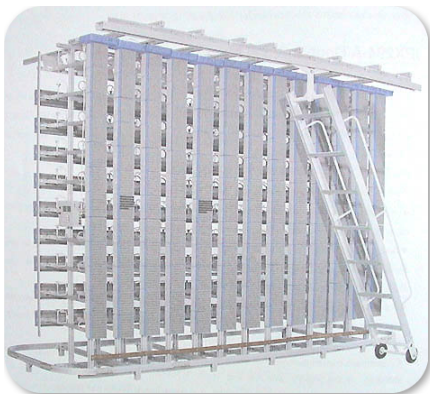
High Density Main Distribution Frame Item Code: STHMDF
