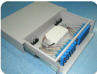
Fiber Optic Splice Patch Panels 12~72 Core Drawer Type Item Code:STFU06
