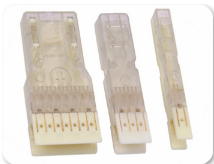
110 Patch Plug 1 Pair 2 Pair 4 Pair Item Code: ST110PP
